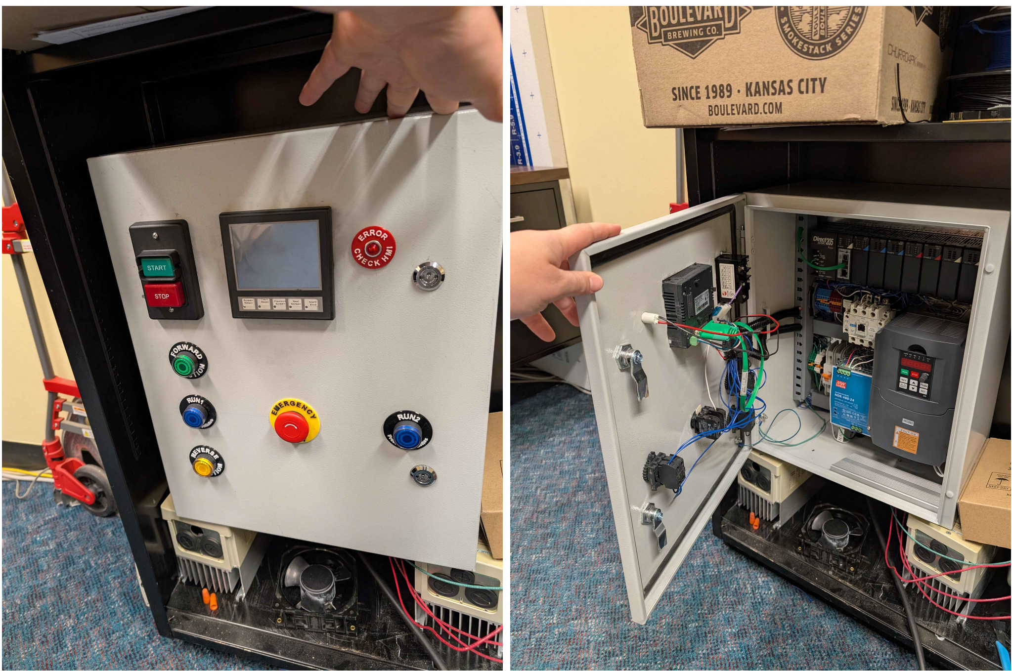
As-built operator face (left) and panel interior (right): EA1-T4CL HMI, deadman / forward / reverse / E-stop, DirectLOGIC 205 rack, Huanyang VFD, 24 VDC supply, SD-N35 contactor, and fused terminal blocks.
